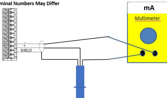
Controller Analog Input Terminals; Actual Terminal Numbers May Differ
