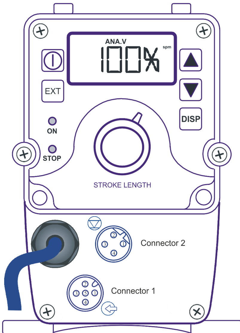
EWN-R Pump
