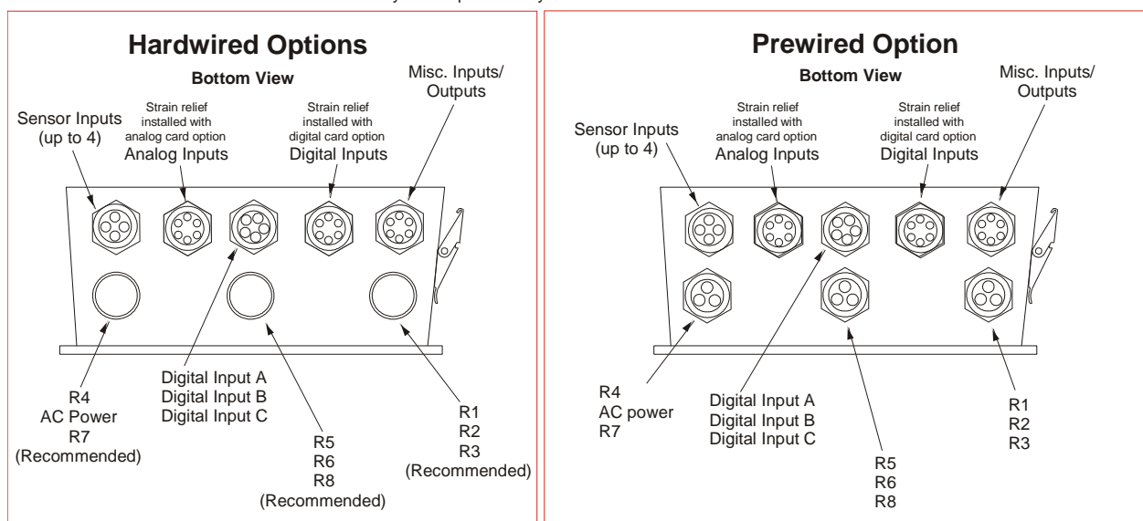
Figure 2: Conduit/Wiring Configuration
