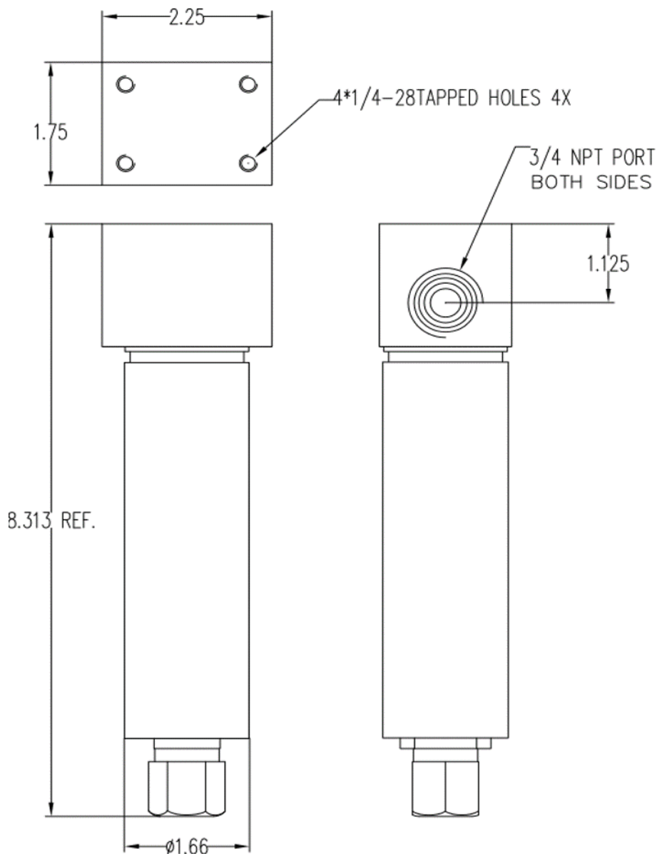
Figure 1. Dimension of the ST-540SS / ST-540SS-N
