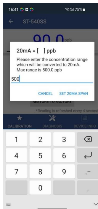
Figure 7. Enter NDSA concentration to set 20mA
