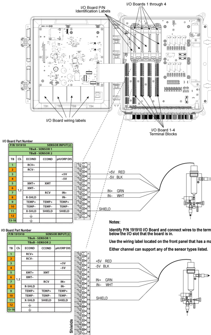
Part Number 191910 Dual Sensor Board Wiring - Disinfection
