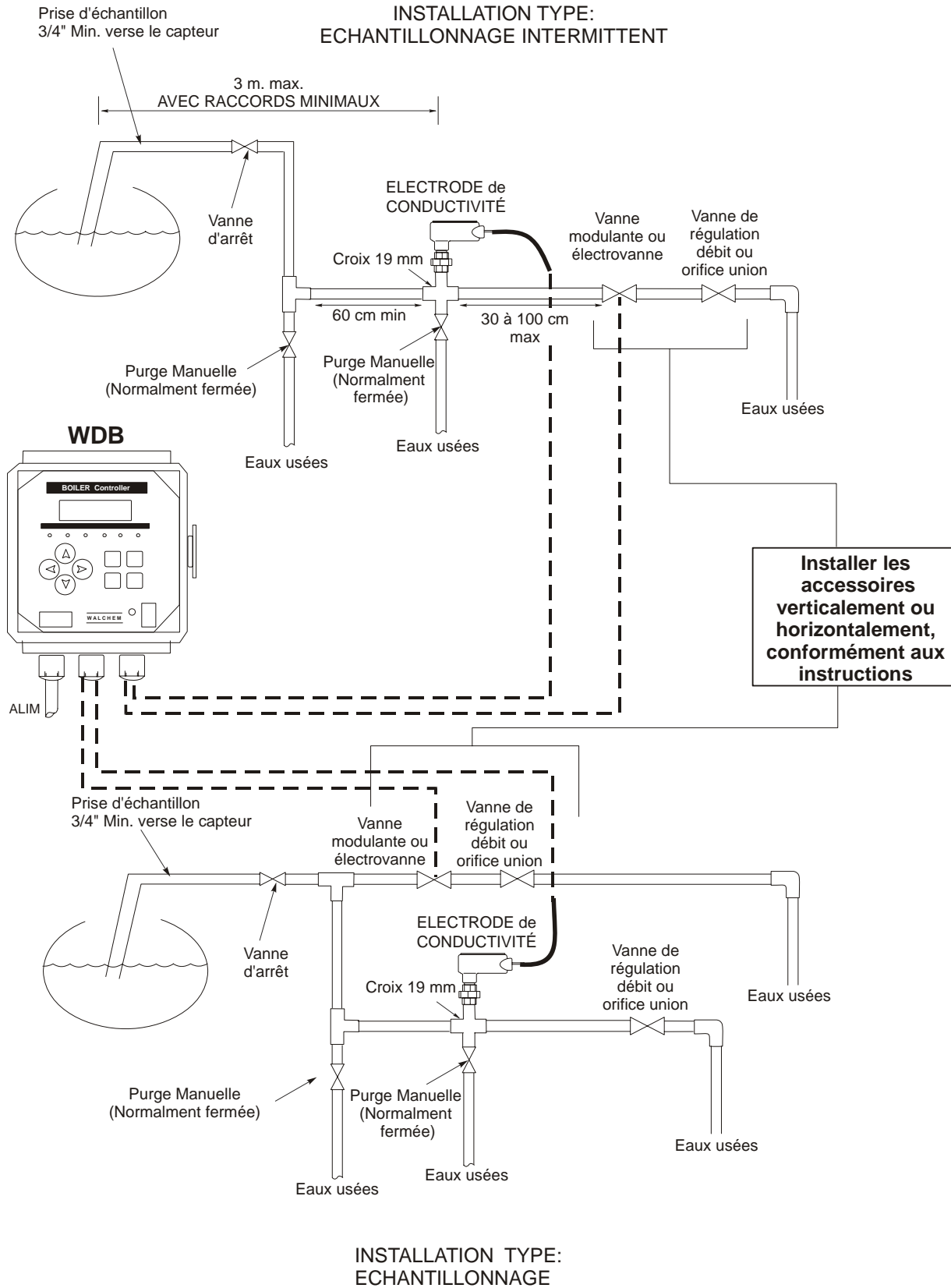
Figure 1 Installation typique
