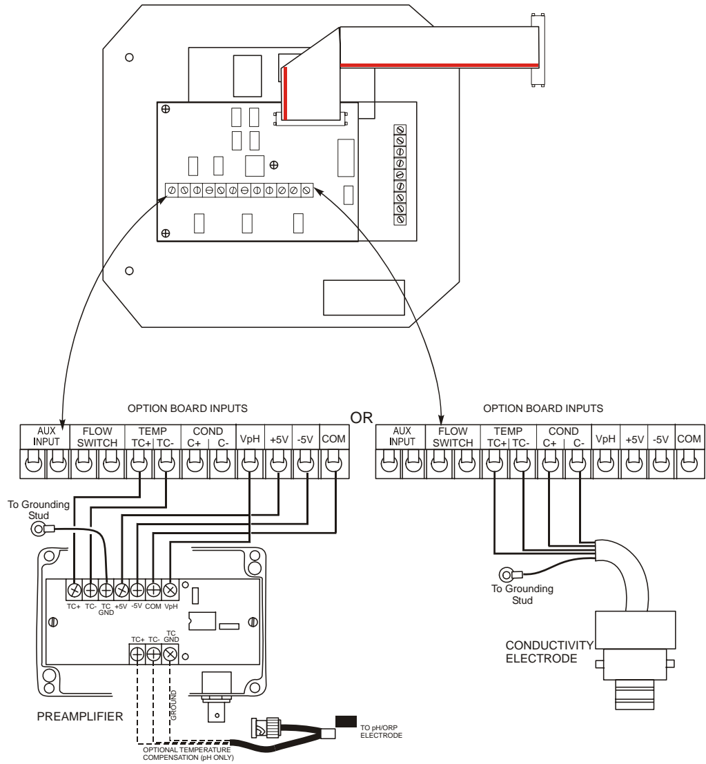
CONNECTIONS SHOWN FOR pH INPUT
